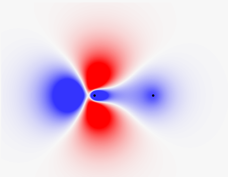
Figure 3.2: The difference density from an excited state of carbyne. This shows that the electron density has moved from around the lone pair on the carbon atom (deep blue), to the bond area.
